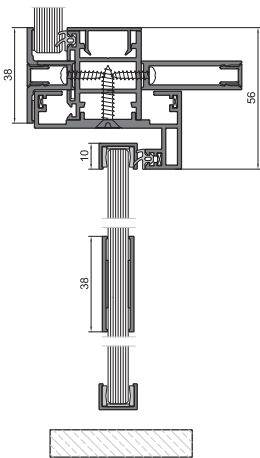
Vertical cross-section - side-hung doors
