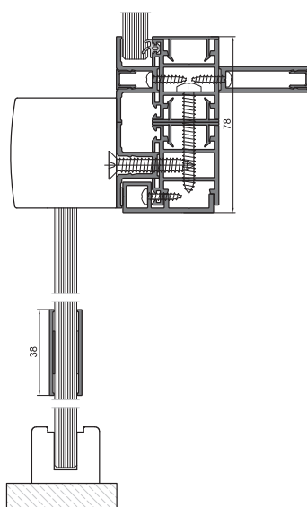
Vertical cross-section - sliding doors
