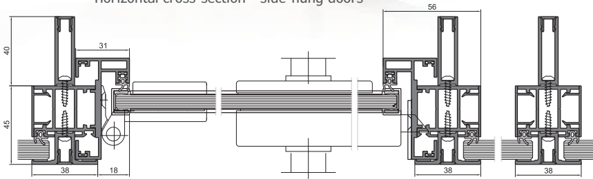
Horizontal cross-section - side-hung doors
